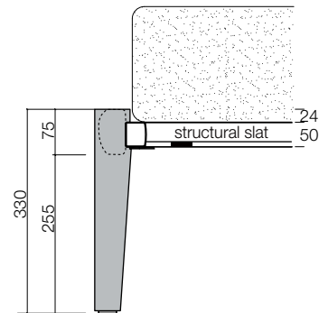
SHAPED bed frame section WITH FOOT
