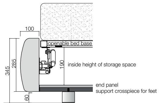
Bed frame section H 285 with STORAGE SPACE
