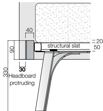
Bed frame section H 90 WITH FOOT -V- IN SHAPED METAL
