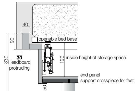
Bed frame section H 90 with STORAGE SPACE
