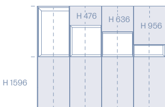
① Moduli L/W 350/725 / Units L/W 425/875 L/W 475/975 L/W 575/1175
