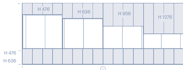
① Moduli L/W 1325/1475/1775/1975 / Units /2075/2175/2375
