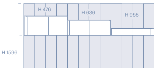
① Moduli L/W 1325/1475/1775/1975 / Units /2075/2175/2375
