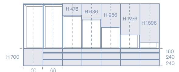
① Moduli L/W 350/725 / Units L/W 425/875 L/W 475/975 L/W 575/1175 ② Moduli cassetti / Drawer units L/W 475/975 L/W 575/1175
