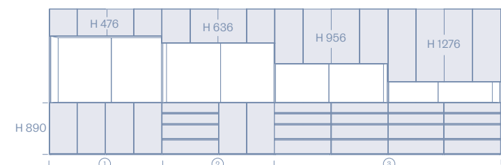
① Moduli / Units 1325/1475/1775/1975 /2075/2175/2375 ② Moduli cassetti e ante / Drawer and door units L/W 1475/1775/1975 /2075/2175/2375 ③ Moduli cassetti / Drawer units L/W 1975/2375
