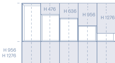
① Moduli L/W 350/725 / Units L/W 425/875 L/W 475/975 L/W 575/1175
